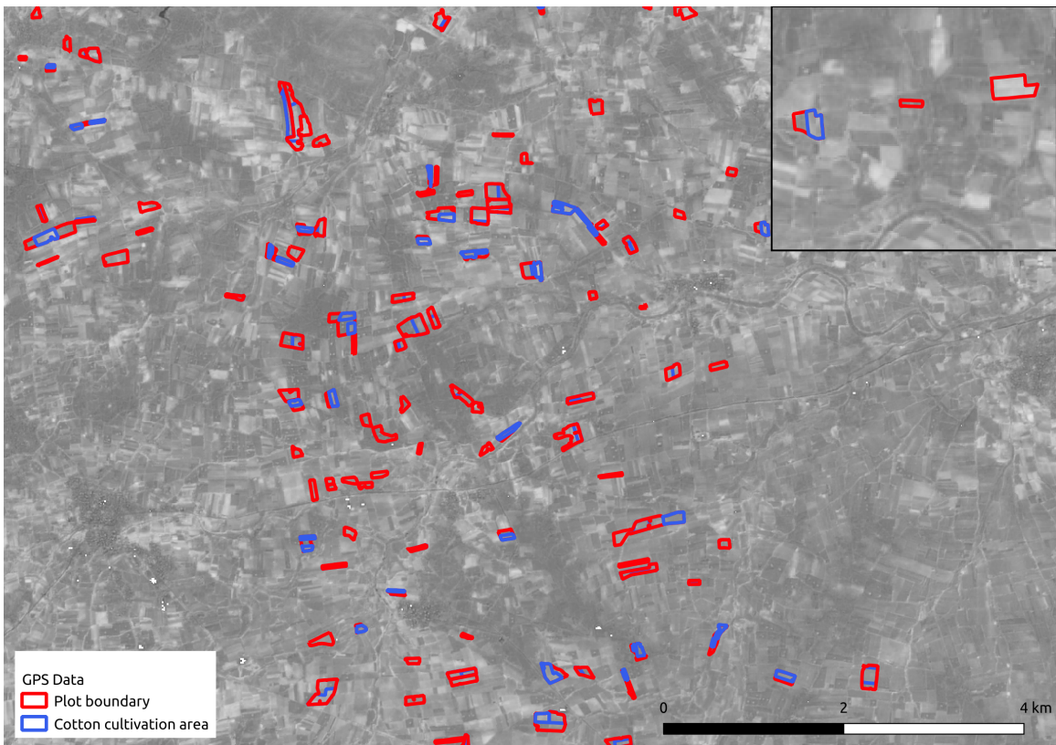
Figure 1 presents sample Sentinel-2 imagery collected on October 28th, 2018 in a portion of the sample region that was selected due to a high density of sample plots. Panel (a) presents a true color composite. Panel (b) presents a reNDVI image, which is the vegetation index used for satellite productivity measurements in this paper. Polygons in red represent the boundaries of sample plots. Polygons in blue show the area on which the farmer cultivated cotton, if they did not cultivate cotton on their full plot.
