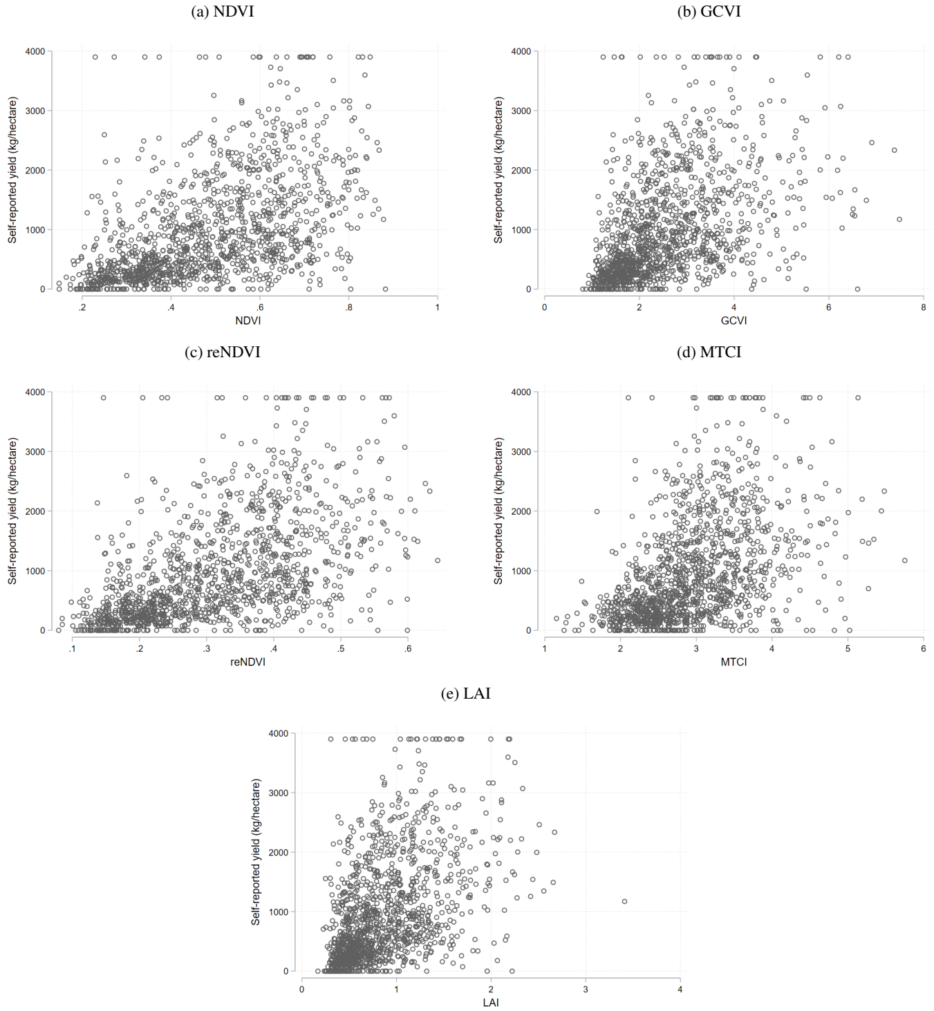
Figure 6 plots vegetation index (VI) values against farmer-reported productivity. We calculated VI values by taking the median value of each VI pixel contained in each sample plot for 5 Sentinel-2 images from 2018. We then took the maximum value across the 5 satellite images. Farmer-reported yield was calculated by taking farmer-reported total harvest data and dividing it by GPS-measured plot area. Positive farmer-reported yield values were winsorized at the 2nd and 98th percentiles.
