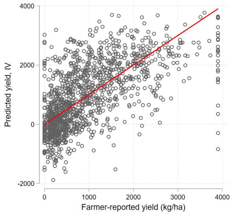
Figure 7 plots farmer-reported yields against satellite yield predictions calibrated using an OLS first stage and a 2SLS first stage. The red line is at 45 degrees. Farmer-reported yield was calculated by taking farmer-reported total harvest data and dividing it by GPS-measured plot area. Positive farmer-reported yield values were winsorized at the 2nd and 98th percentiles.
